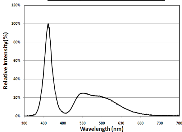
Wavelength vs. Relative Intensity
