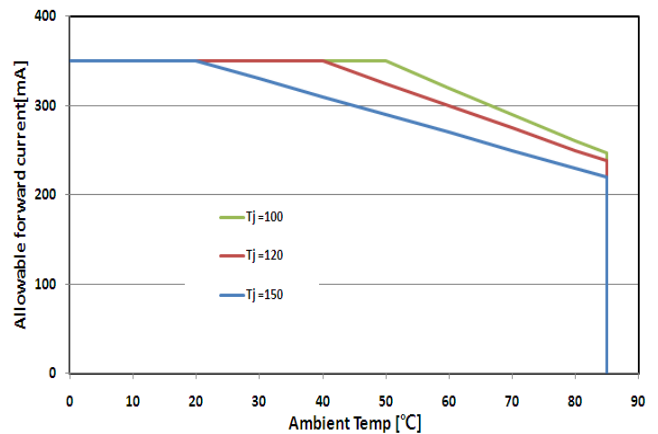
Ambient Temp. vs. Allowable forward current
