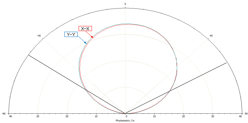
Radiation Characteristic @25°C (120mA)
